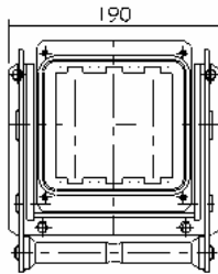
129/12/400-1 3-way Bulkhead Plug
