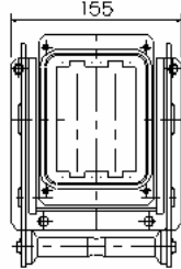
129/12/401-1 2-way Bulkhead Plug
