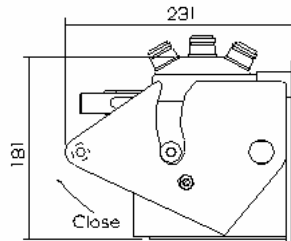
Vertically Mounted Plug & In-line Socket
